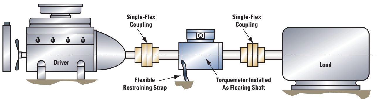
Figure 1. Floating Shaft Mount
